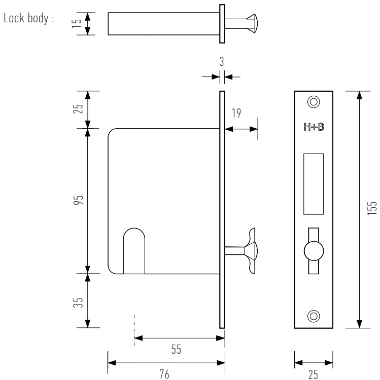
Shown with HB 660 Flush Pull (ordered seperately)
