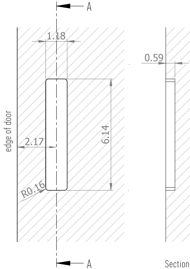
Milling Drawing for timber doors with fixing kits
