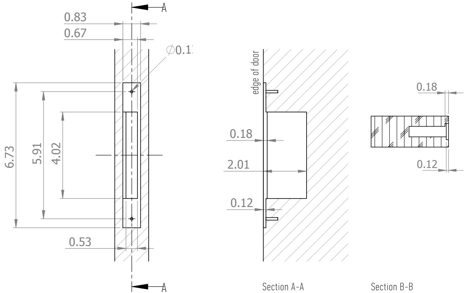
Milling Drawing for timber doors
